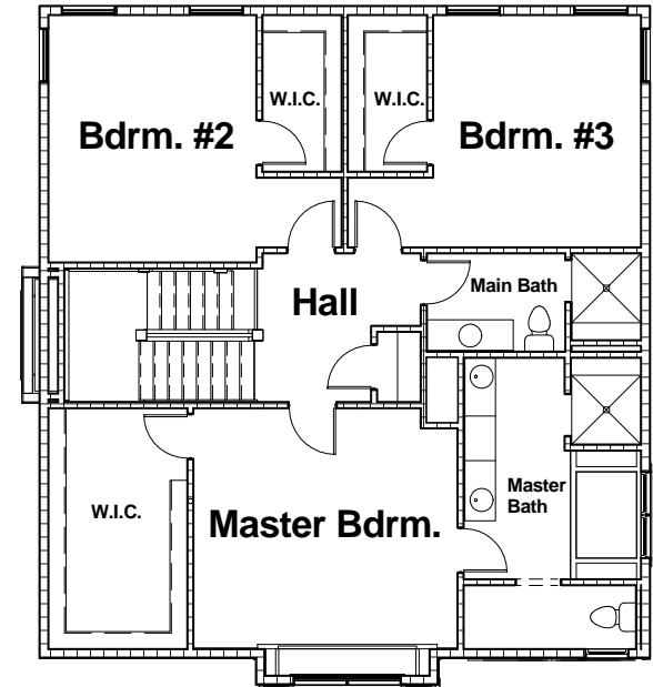
② Second Floor 1 : 148
