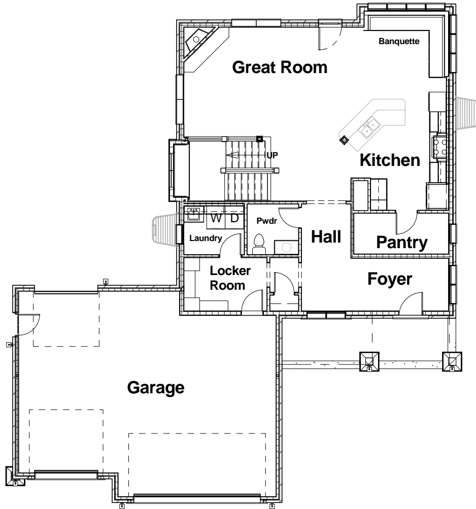
① First Floor 1 : 148
